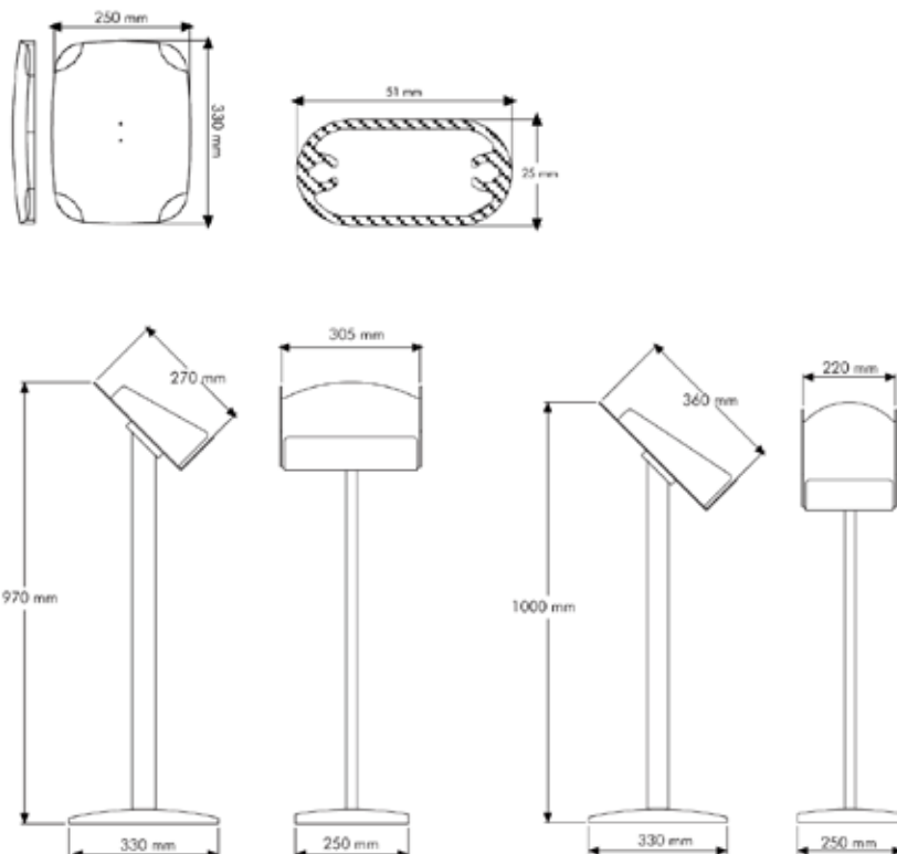
Decorative base powdercoated 9006 1,62 kg
